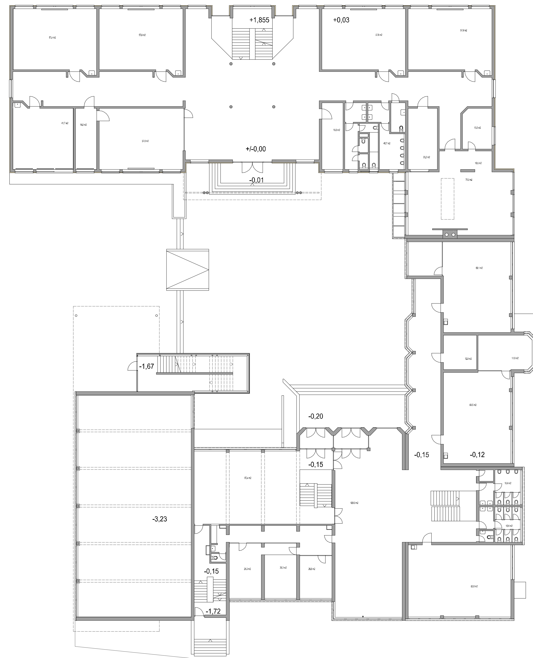
Erdgeschoß 969 m2
